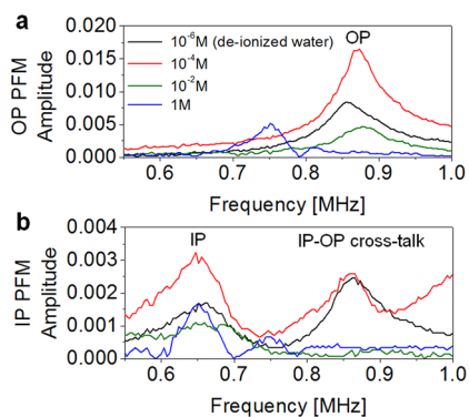
Figure 1. (a) OP and (b) IP PFM amplitude as a function of excitation frequency for Na 2 SO 4 electrolytes with molarities from 10 -6 to 1 M.
