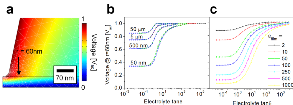
Figure 6. (a) Voltage distribution near the tip apex for an electrolyte \tan \delta = 14 and a film thickness 50 nm when 1 V_{ac} is applied to the tip. (b) Numerically obtained absolute values of the potential on the film surface at a distance from the tip r = 60 nm vs electrolyte loss tangent for film thicknesses, as indicated at the curves in the plot. The film dielectric constant is 107. The simulations were performed for four driving frequencies: 6.5 kHz (black), 65 kHz (red), 650 kHz (green), and 6.5 MHz (blue). Tip apex radius is 30 nm. (c) Absolute values of the potential on the film surface at a distance from the tip r = 60 nm vs electrolyte conductivity for a film thickness of 50 nm and different values of the film dielectric constant as indicated in the plot.
