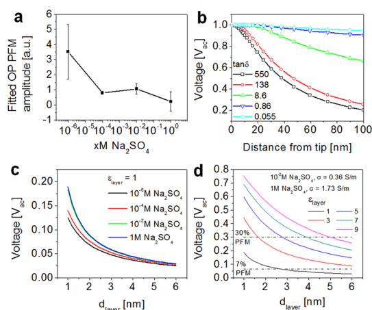
Figure 5. (a) OP PFM amplitude extracted from multifrequency detection methods as a function of molarity with a molarity of 10^{-6} for deionized water. (b) Voltage under the biased SPM tip as a function of radial distance for electrolytes with various \tan \delta when 1 V ac is applied to the tip. (c) Effective voltage on the sample surface underneath the tip as a function of dead layer thickness, d_{\text{layer}} for a dielectric constant of the dead layer of \epsilon_{\text{layer}} = 1 for solutions of different conductivities. (d) Effective voltage on the sample surface underneath the tip as a function of dead layer thickness, d_{\text{layer}} for 1 M Na 2 SO 4 for various values of \epsilon_{\text{layer}} . The effective voltages on the sample are indicated for 10^{-2} M Na 2 SO 4 and 1 M Na 2 SO 4 as estimated from (a) relative to the measurement in deionized water.
