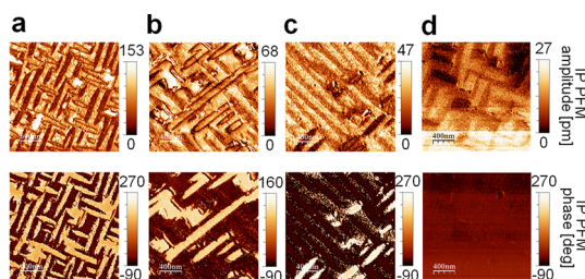
Figure 2. IP PFM images for BFO measured in a liquid environment at 650 kHz in (a) 10 -6 M Na 2 SO 4 , (b) 10 -4 M Na 2 SO 4 , (c) 10 -2 M Na 2 SO 4 , and (d) 1 M Na 2 SO 4 .
