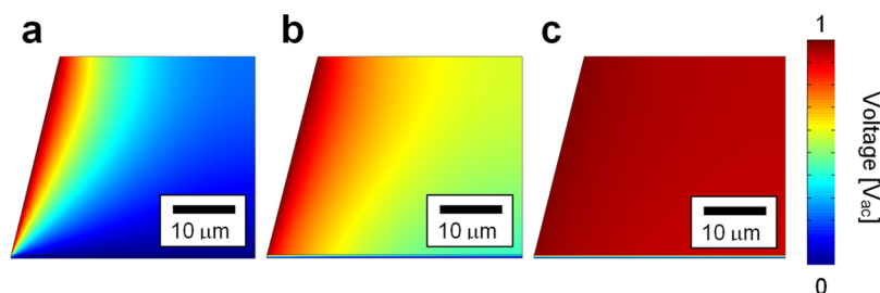
Figure 4. Numerically obtained voltage distributions when 1 V ac is applied to the tip for the following electrolytes: (a) deionized water ( s = 1.5 \times 10^{-4} S/m, \tan \delta = 5.2 \times 10^{-2} ) and 10^{-4} M Na 2 SO 4 solution ( s = 2.6 \times 10^{-3} S/m, \tan \delta = 0.9 ); for these solutions, the potential distributions are indistinguishable at the length scale of the plot; (b) 10^{-2} M Na 2 SO 4 solution ( s = 0.36 S/m, \tan \delta = 124 ); (c) 1 M Na 2 SO 4 solution ( s = 1.73 S/m, \tan \delta = 590 ).
